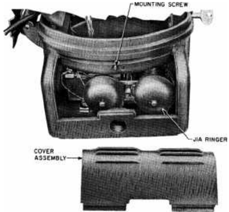
Fig. 12—525-Type Outdoor Telephone Set, Lower Cover Assembly Removed
