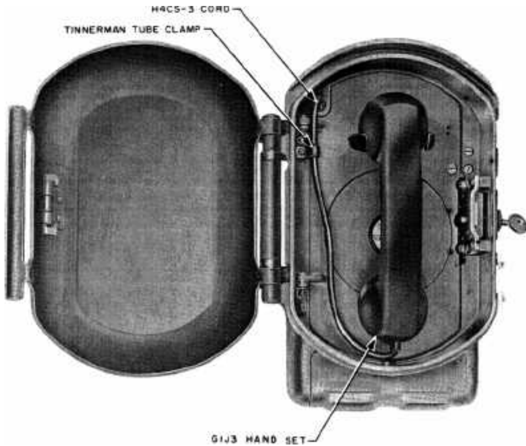
Fig. 9—525A Outdoor Telephone Set (Manual)
