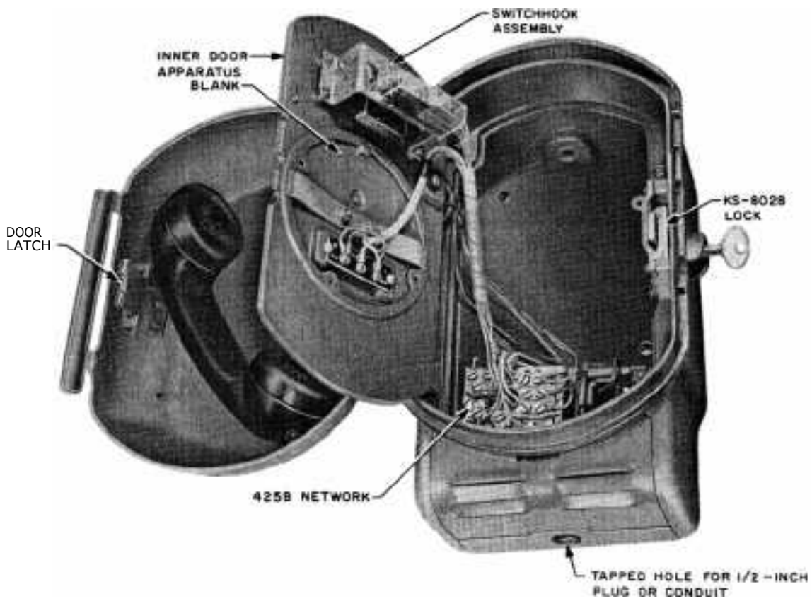
Fig. 11—525A Outdoor Telephone Set (Manual), Inner Door Open
