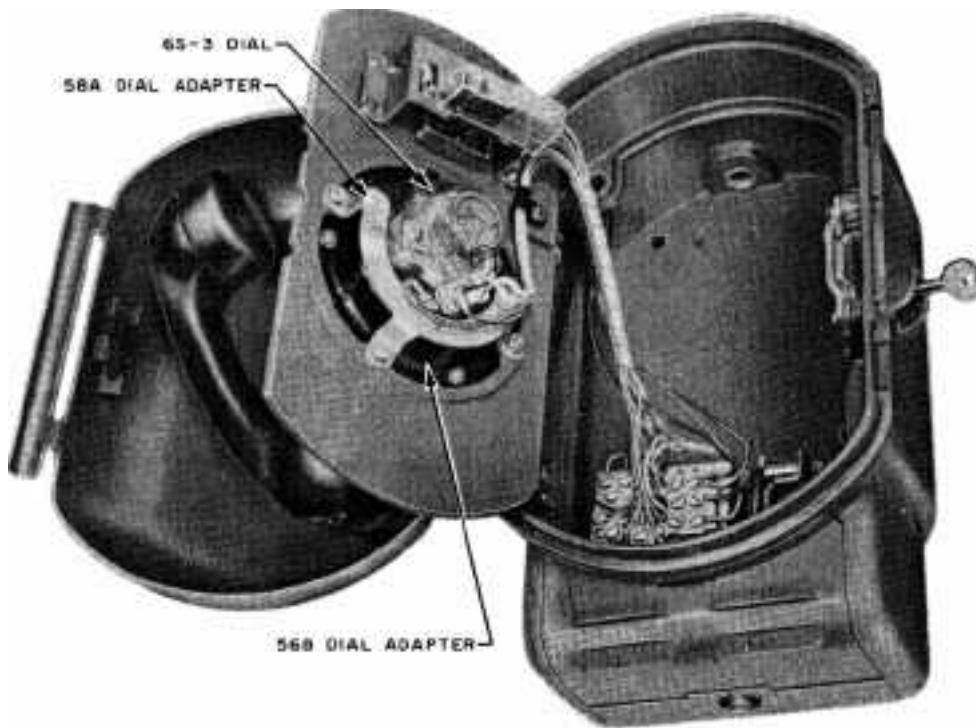
Fig. 10—525B Outdoor Telephone Set (Dial), Inner Door Open
