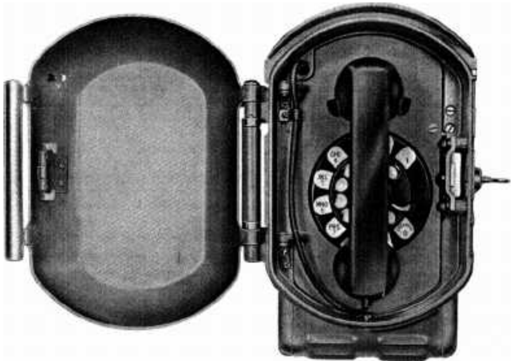
Fig. 8—5258 Outdoor Telephone Set (Dial)
