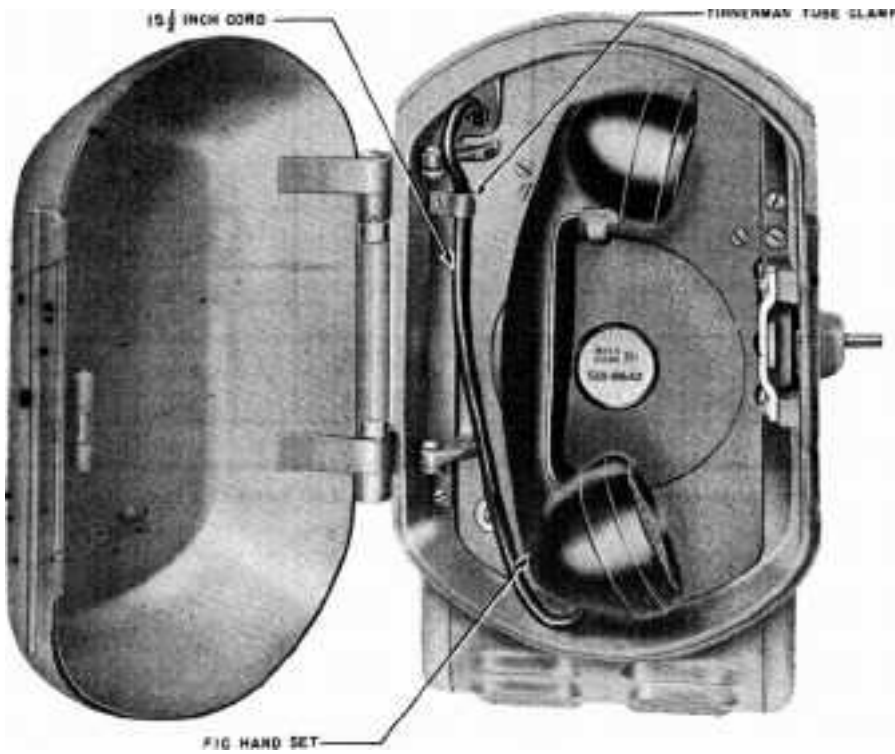
Fig. 3—325-Type Outdoor Telephone Set, Manual
